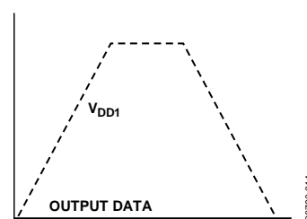
Figure 14. V_{DD1} Power-Up/Power-Down Characteristics, Input Data = Low
